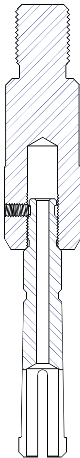
Standing Valve Retriever
