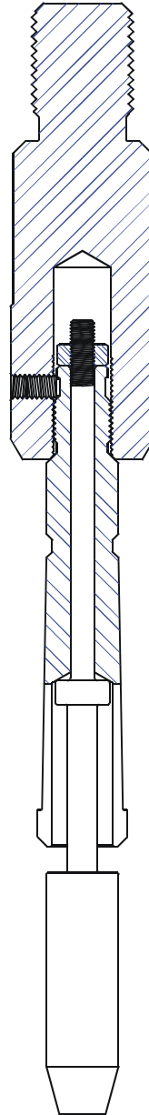
Standing Valve Retriever w/ Knock-out Bar
